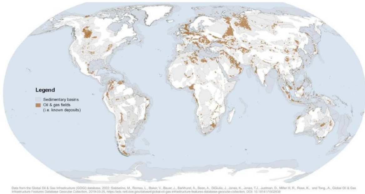
Figure 3. Sedimentary basins and oil and gas fields (i.e. known fossil fuel deposits).
