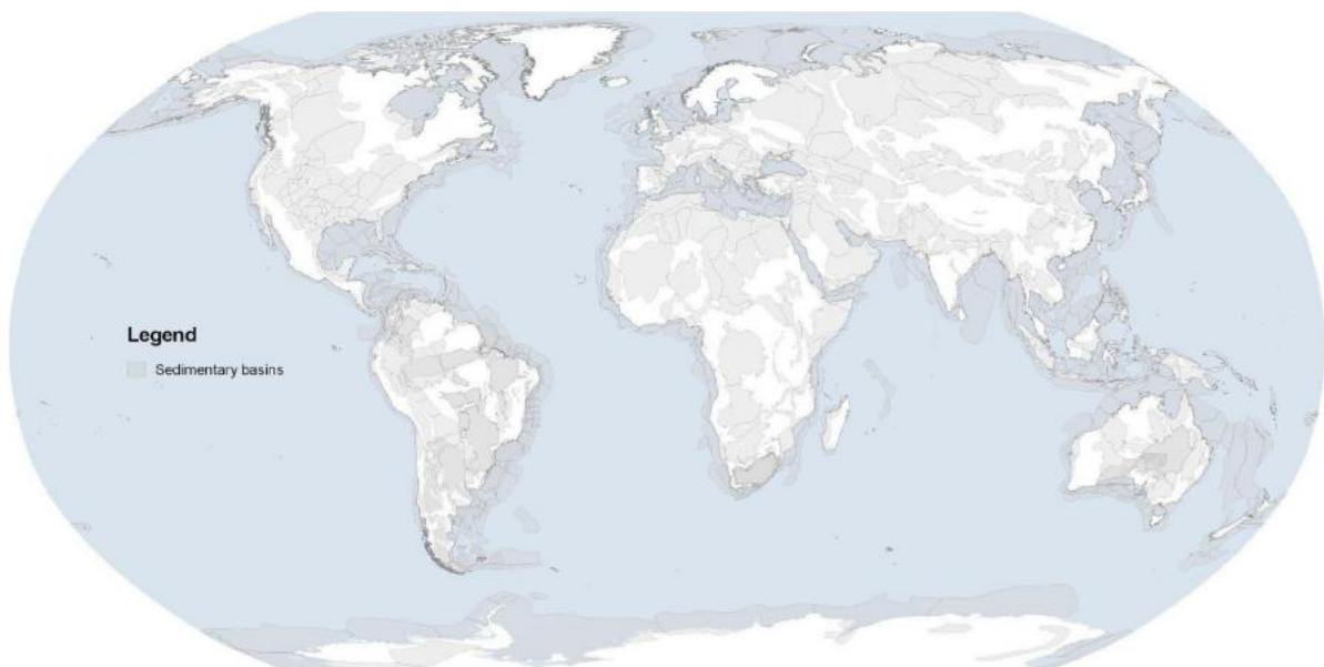
Figure 2. Earth's sedimentary basins. Sedimentary basins are areas of earth's crust where organic material and sediment have collected and compacted over millions of years, sometimes in conditions that form hydrocarbon deposits.
